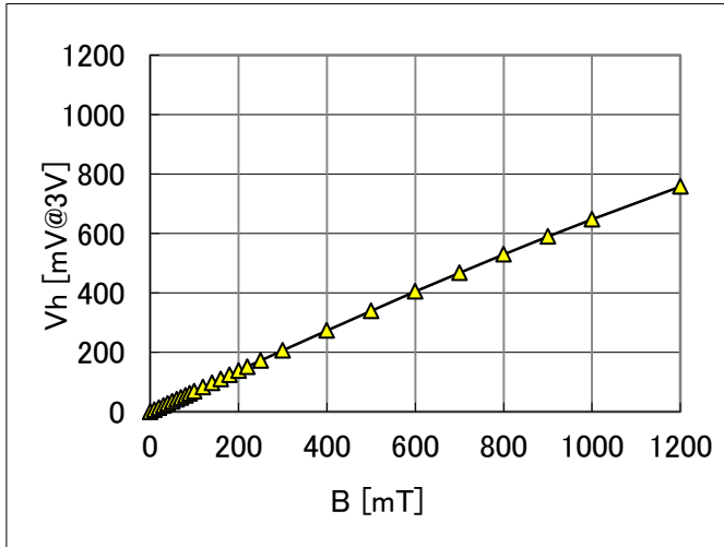
●Constan Vltage drive@3V
