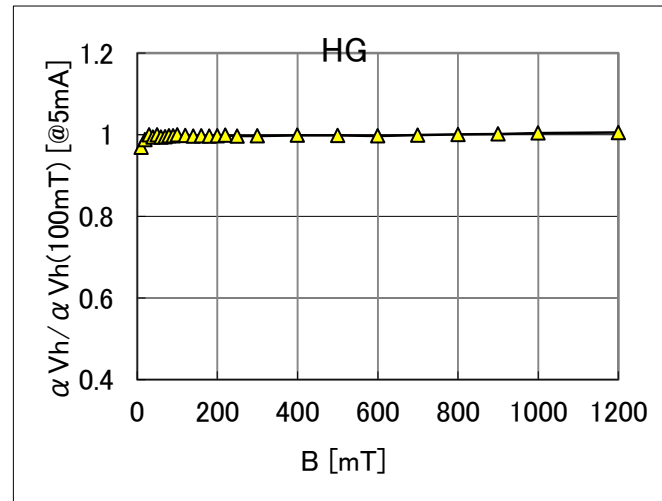
●Consyant Current drive@5mA
