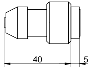
MATING CONNECTOR AMPHENOL SOCKET 62GB-16J10-7S WITH SHROUD
