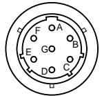
AMPHENOL FIXED PLUG 62GB-51T10-7P
