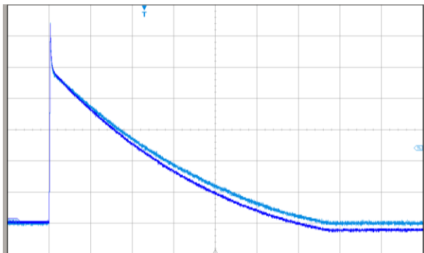
Ch 1: Co-axial shunt - DC-800MHz – 16.2mV/div Ch 2: CWTMiniHF 3 - 250mV/div (25A/div) – LF(-3dB) 11Hz Time base: 200µs/div
