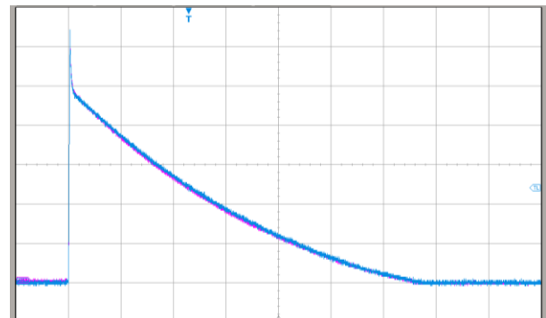
Ch 1: Co-axial shunt - DC-800MHz – 40mV/div Ch 3: CWTMiniHF 3 - 250mV/div (25A/div) – LF(-3dB) 2.3Hz Time base: 200µs/div
