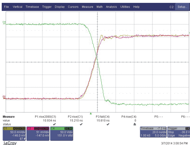
Figure 4: Comparison of reference and Rogowski probe measurements. Time base 20ns/div C2 - CWTMini/03 (Note the waveforms include 16.8ns de-skewing to eliminate the inherent yet predictable delay of the Rogowski current transducer. This delay is the sum of delay in the Rogowski coil, the connecting cable and the integrator)
